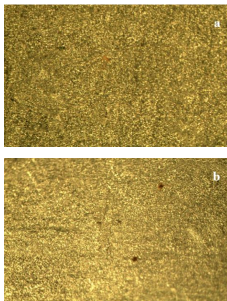
Fig. 2 Stereoscopic magnifying glass image for the AR condition, considering different exposure times to the salt spray: a) 8 h and b) 96 h. M [4.5x].
