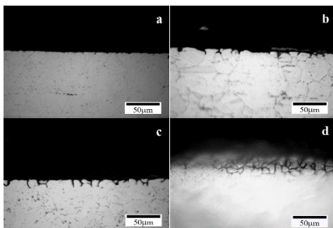
Fig. 6 Intergranular corrosion path in as-received and heat treated AISI 316L considering different exposure times to the saline solution. a) As-received (50h), b) As-received (96h), c) Heat treated (8h) and d) Heat treated (96h).
